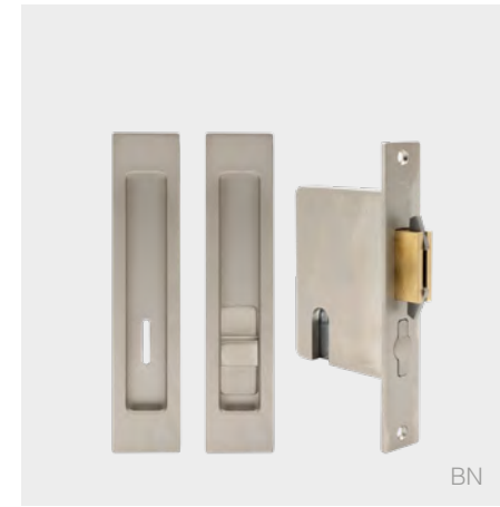
690 170mm x 36mm 55mm b/s Minimum thickness 38mm Please use 690/35 for 35mm thickness
